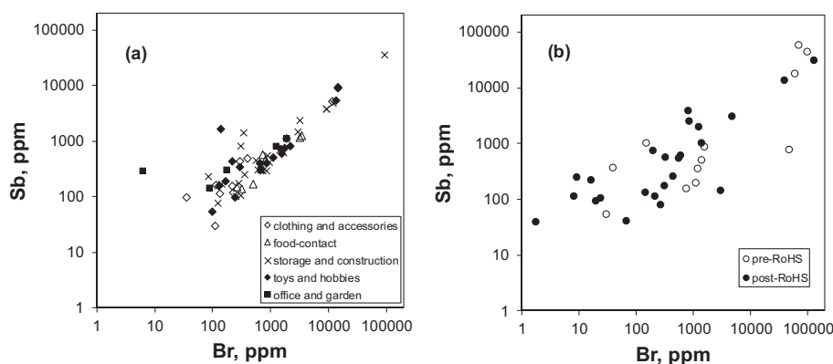
Fig. 2. Concentrations of Sb versus concentrations of Br in non-EEE black plastic samples (a) and black plastic EEE casings (b).
