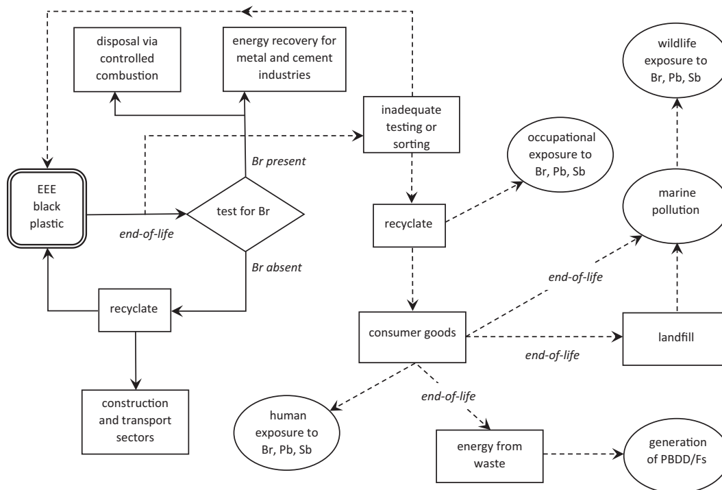
Fig. 4. The life cycle of black plastic used in EEE. Solid lines represent the preferred pathways based on adequate testing for Br, while broken lines represent the non-preferred pathways along with exposure routes and environmental impacts of hazardous additives (brominated compounds, Pb and Sb).
