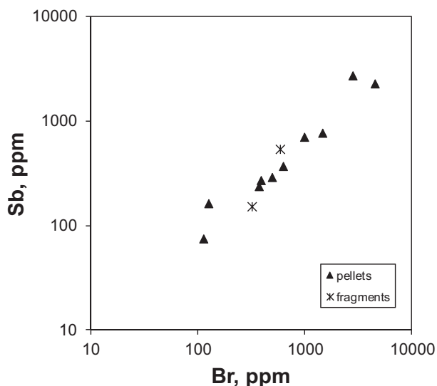
Fig. 3. Concentrations of Sb versus concentrations of Br in beached black plastics. Note that Sb was not detected in distinct objects that were non-PVC-based.
