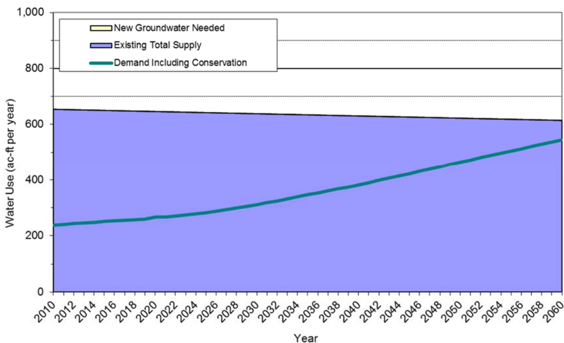
Figure 6-5 Wahweap Creek Subbasin Supply and Demand
