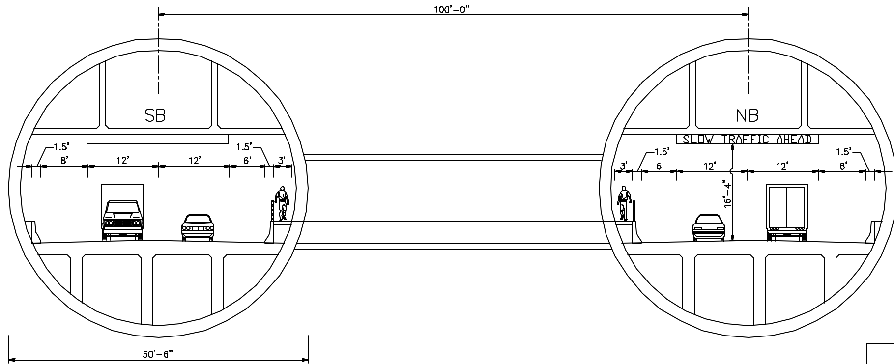
TWIN TUNNEL CROSS SECTION
