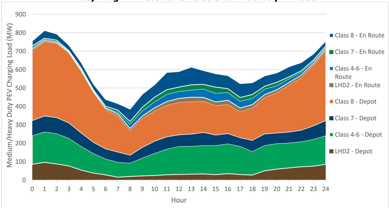
Figure 4: Projected Statewide Charging Demand for 155,000 Medium- and Heavy-Duty Plug-In Electric Vehicles on a Weekday in 2030
