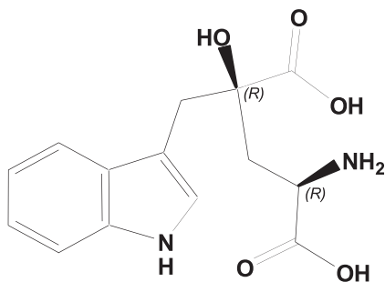
Fig. 1. The 2 R ,4 R -isomer of 2-hydroxy-2-(indol-3-ylmethyl)-4-aminoglutaric acid.
