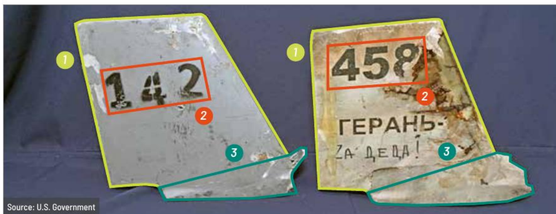
Left: A Shahed-131 wing stabilizer recovered from an attack in Iraq that Iran claimed, September 2022 Right: A Geran-1 wing stabilizer recovered in Ukraine, fall 2022
