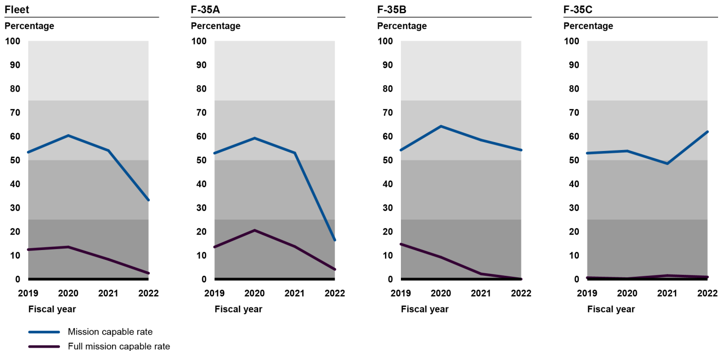
Figure 16: Performance of F-35 Aircraft Built between 2008 and 2011, Fiscal Years 2019 through 2022
