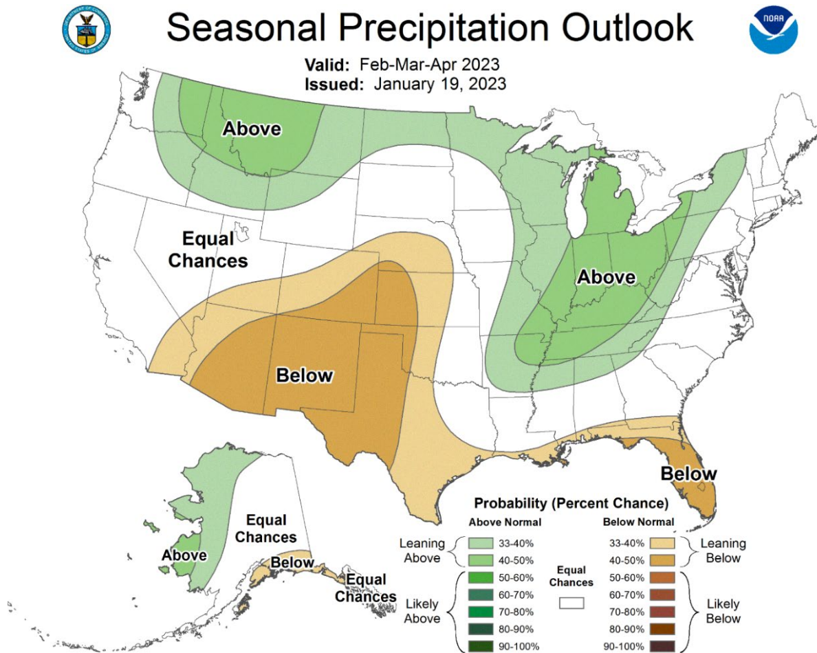
Figure 1-2 NOAA seasonal precipitation outlook (issued in January 2023).
