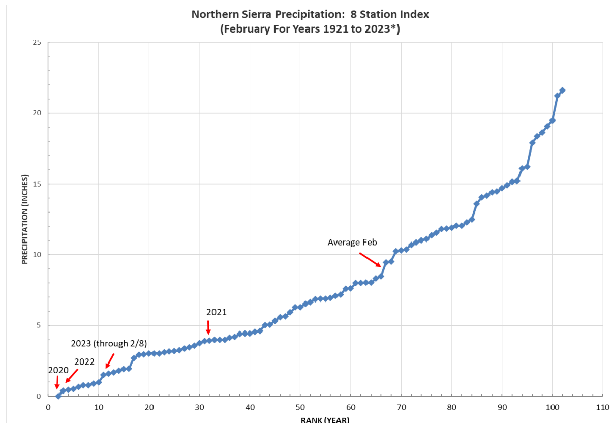
Figure 1-1 Ranking of historical February Northern Sierra 8-Station Index precipitation.
