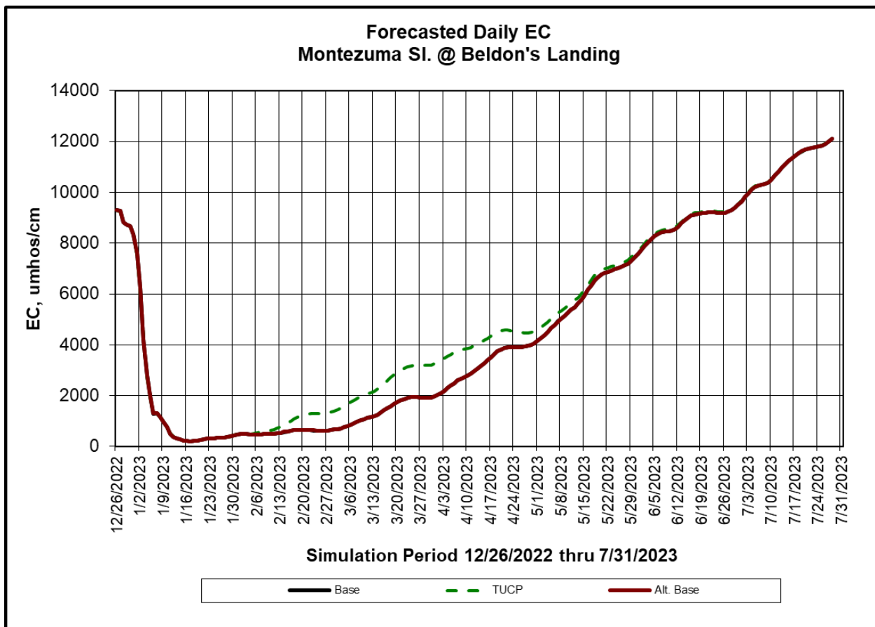
Figure DS3. Daily Electrical Conductivity in Montezuma Slough at Beldon’s Landing from DSM2 Modeling.
