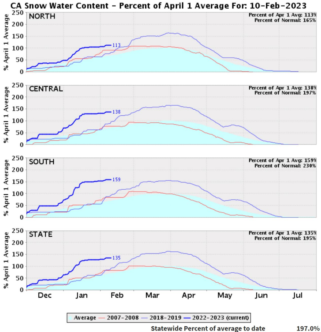
Figure 1-3 Progression of snow water content for Water Year 2023 as compared to Water Year 2008, Water Year 2019, and long-term average.
