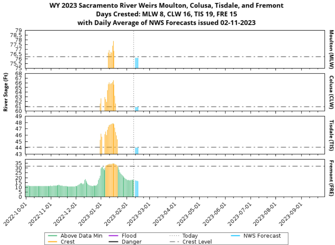
Figure WR5. Sacramento Weir Overtopping periods, October 2022 through February 11, 2023.
