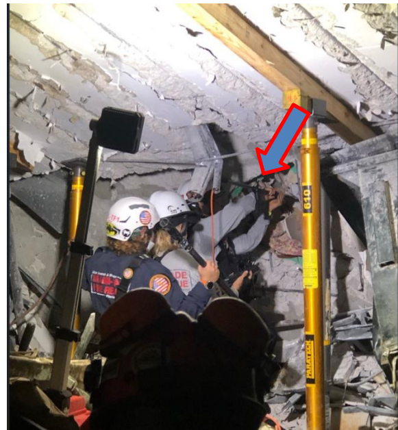
Image 4: Search camera used to view behind the slab.
