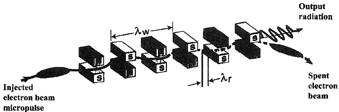
Figure 8. Free-Electron Laser Wiggler
