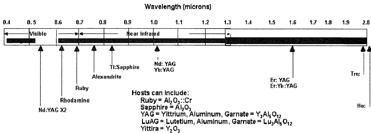
Figure 5. Common Solid-State Lasers and Their Wavelengths
