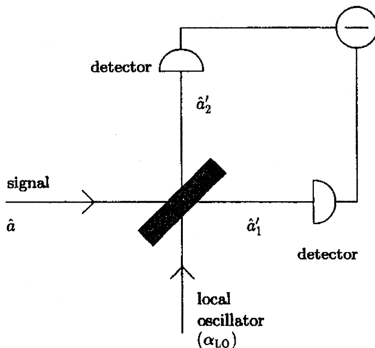
Figure 10. Schematic of a Balanced Homodyne Detector. (courtesy of Ulf Leonhardt)
