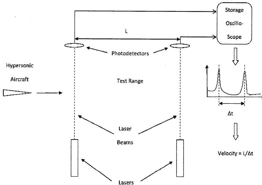
Figure 8. Laser-Based Chronograph.
