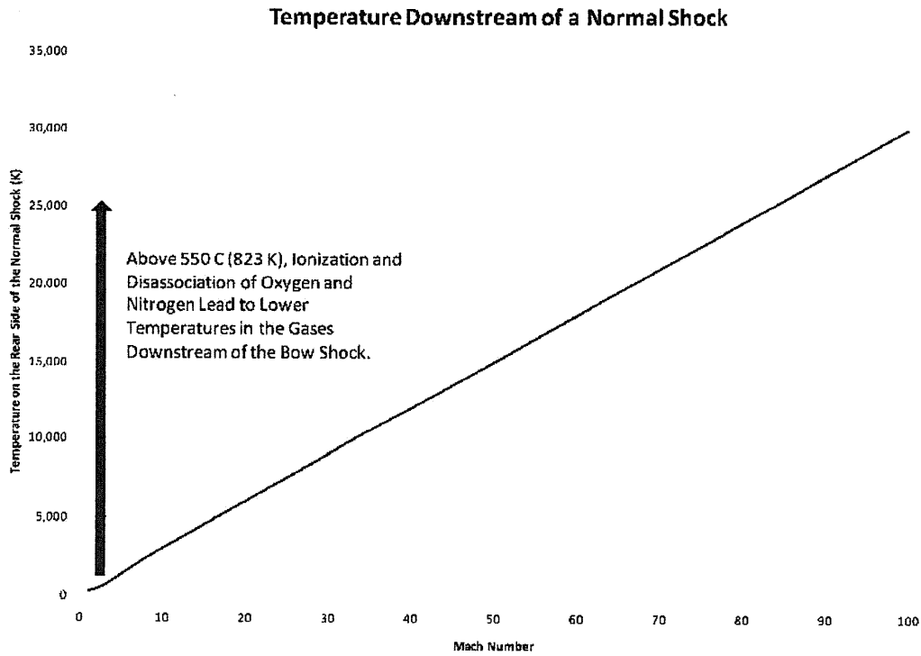
Figure 16. Peak Shock Layer Temperature for Hypersonic Objects.
