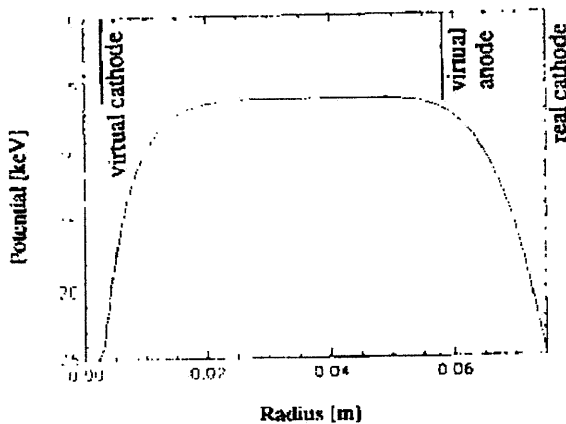
Figure 4.7. The Double Well Potential Calculated With IXL Code for d_{33perp} , i=14\text{keV} , I_i=55\text{A} , I_e=59\text{A}
