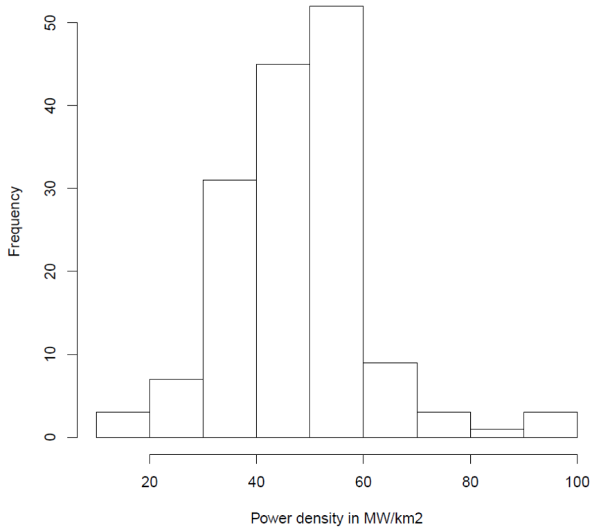
Histogram of the power densities of systems reporting a nameplate capacity of >= 5MW
