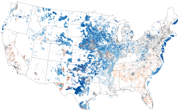
(a) RE+ (100% renewables) scenario, Base land use assumptions (BLUA)
