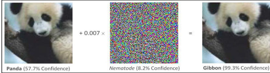
Figure 1. AI Failure in Image Recognition
