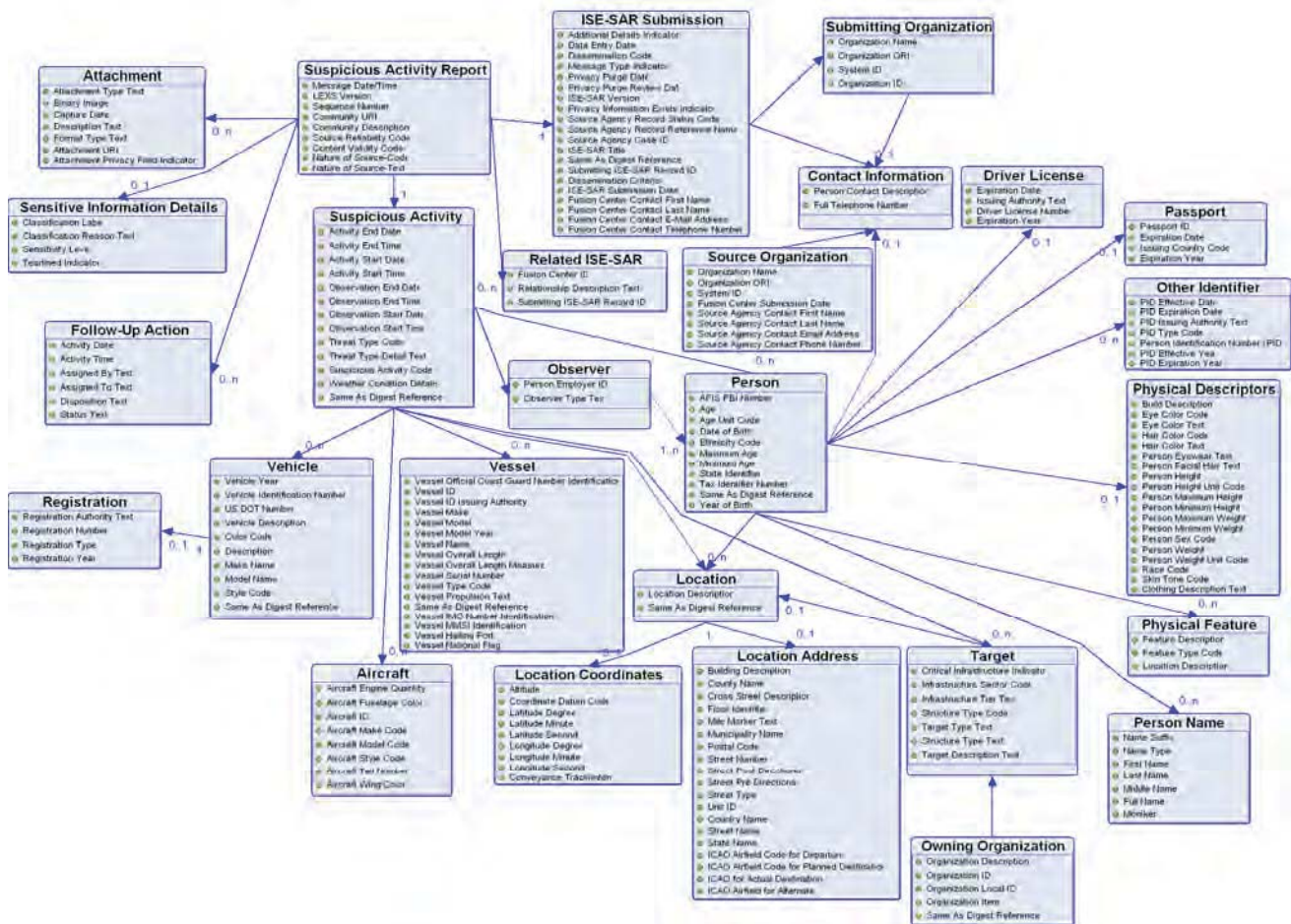
Figure 2 – UML-based Model
